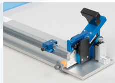
vertical adjustment
